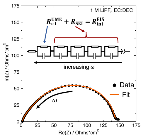
Figure 5. Transient CV can calculate the contribution of the electron transfer resistance to the total impedance of lithium anodes. EIS data of a symmetric Li || Li cell with LiPF 6 in EC:DEC electrolyte. The data is fit to an equivalent circuit, 58 shown as an inset, where the first R/C circuit represents the electron transfer (calculated from transient CV), and the second to fifth R/C circuits represent the impedance of the SEI. 5,7,29,58
