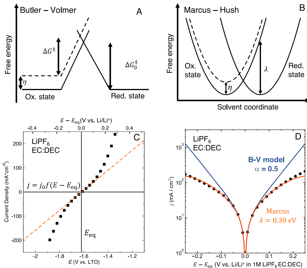
Figure 2. Marcus models of charge transfer accurately describe the electron transfer kinetics of the Li/Li + redox couple, while the Butler–Volmer model fails when E - E_{\text{eq}} > |\pm 50 \text{ mV}| . (A) Schematic of the potential energy surface in the Butler–Volmer model. (B) Schematic of the potential energy surface in the Marcus–Hush model. (C) Representative CV data from the box labeled “kinetically controlled region” in Figure 1D. Only the data < 10\% of i_p is included. The dashed orange line is the linear least-squares fit to j = j_0 f(E - E_{\text{eq}}) . (D) Comparison of the Butler–Volmer and Marcus–Hush model for 1 M LiPF 6 in EC:DEC. CV data are the black dots; Butler–Volmer is the solid blue line, and Marcus–Hush is the solid orange line.
