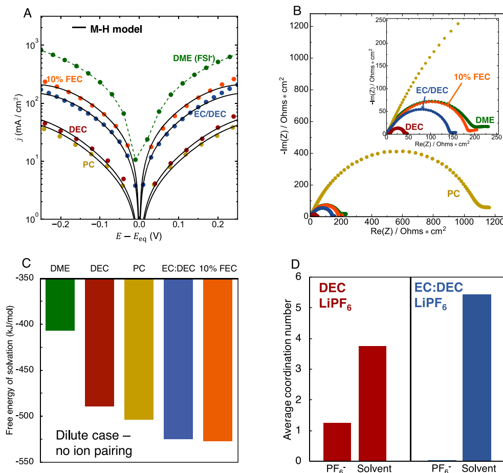
Figure 4. Effect of solvent on the charge transfer kinetics. (A) Tafel plots of LiPF 6 in PC (golden, v = 20 V/s), DEC (red, v = 20 V/s), EC:DEC (blue, v = 10 V/s), EC:DEC + 10% FEC (orange, v = 15 V/s), and DME (green, v = 50 V/s). (B) Corresponding Nyquist plots of Li || Li symmetric cells. (C) Dilute free energy of solvation for Li ions in each solvent calculated from molecular dynamics simulations. (D) Comparison of the average coordination environment of Li ions in DEC and EC:DEC calculated by molecular dynamics simulations.
