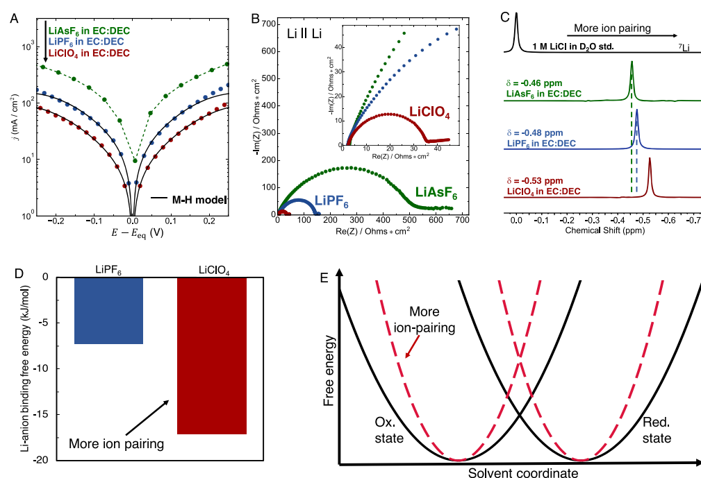
Figure 3. Ionic activity of Li ions dictates the rate of electron transfer in electrolytes with the same solvent. (A) Tafel plots of LiAsF 6 (green, v = 20 V/s), LiPF 6 (blue, v = 10 V/s), and LiClO 4 (red, v = 10 V/s) in EC:DEC. The solid black lines show the corresponding Marcus fits. LiAsF 6 is dashed because the experiment is not under total kinetic control. (B) Corresponding Nyquist plots of Li || Li symmetric cells in each electrolyte. (C) 7 Li NMR spectra. (D) Comparison of the binding free energies of Li ions and each anion in EC:DEC calculated by molecular dynamics simulations. (E) Schematic of the effect of ion pairing on the potential energy surface.
