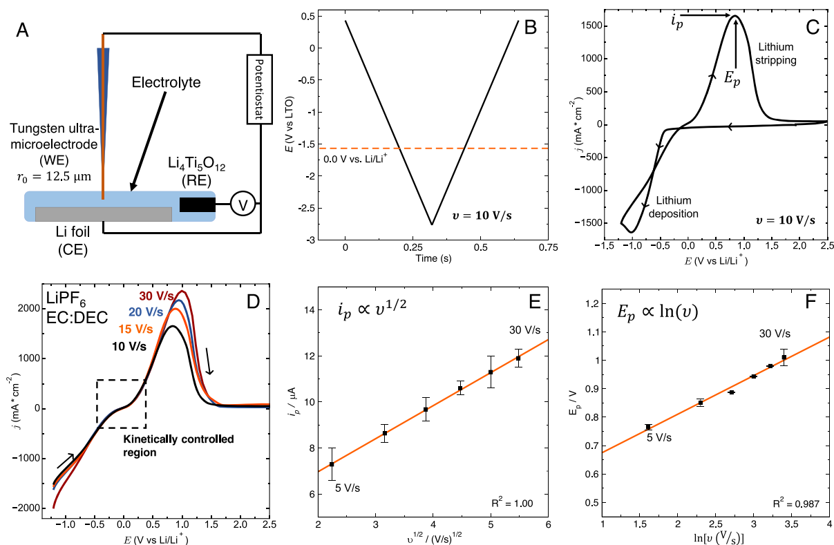
Figure 1. Ultramicroelectrodes can measure the electron transfer kinetics of lithium metal deposition and dissolution. (A) Schematic of the ultramicroelectrode cell. (B) A representative potential profile shows that the experiment is completed in less than one second. (C) A representative full voltammogram for the transient CV in 1 M LiPF 6 in EC:DEC. (D) The reverse sweep of the CV experiment with 1 M LiPF 6 in EC:DEC shows that there is a kinetically controlled region close to the formal potential of lithium. Forward sweeps are removed for clarity. (E) The i_p varies linearly with v^{1/2} , and (F) E_p varies linearly with \ln(v) , which indicates that the CV experiment is fully irreversible— or under kinetic control near the formal potential. Error bars represent the standard deviation of at least three experiments at each scan rate.
